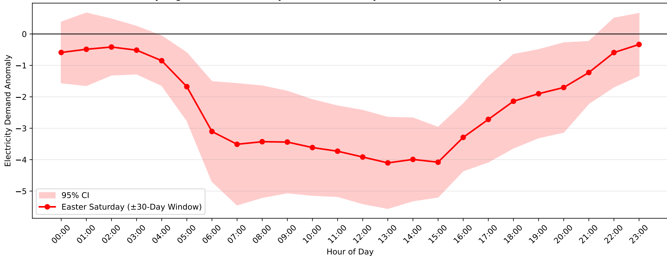
Wyong Demand Anomaly: Easter Saturday (2004–2017, \pm 30 -Day Window)
